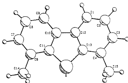
Fig. 3. X-ray crystal structure of 4,6-dimethyldibenzothiophene (8)
