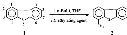
Fig.1. Synthesis of 4-methyldibenzothiophene
